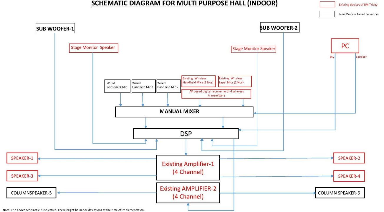
SCHEMATIC DIAGRAM FOR MULTI PURPOSE HALL (INDOOR)
